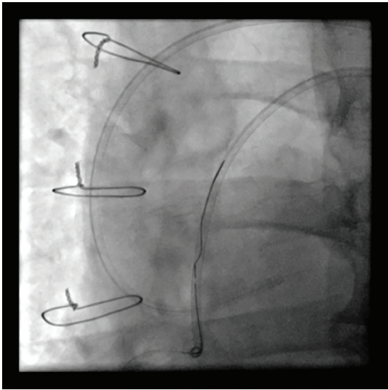
Figure 4. Extrahepatic step
