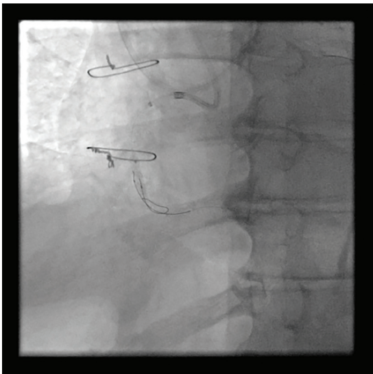
Figure 3. Reverse CART
