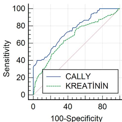
Figure 1. ROC curve
